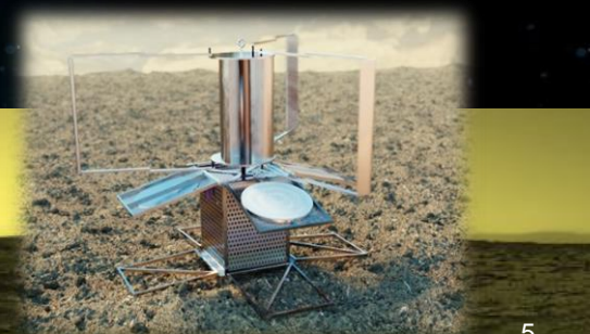
Early LLISSE concept – wind powered
