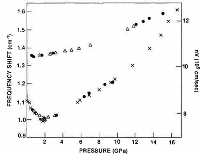
Grimsditch, 1984
