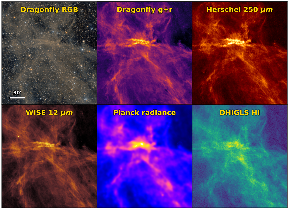
Figure 1: Example dataset of the DGL in different dust tracers. (Liu et al. to be submitted)
